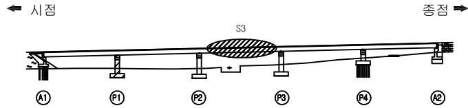
KEY PLAN (종단)
